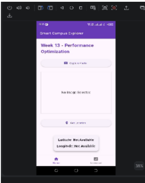
Figure 1: Home screen.
