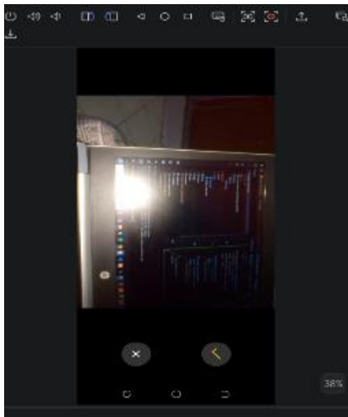
Figure 2: Camera feature.
