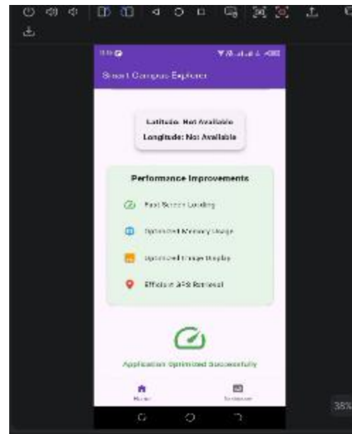
Figure 1: Home screen.
