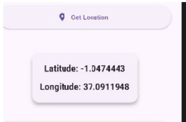
Figure 1: Home screen.
